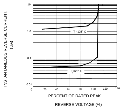
FIG.4-TYPICAL REVERSE CHARACTERISTICS
